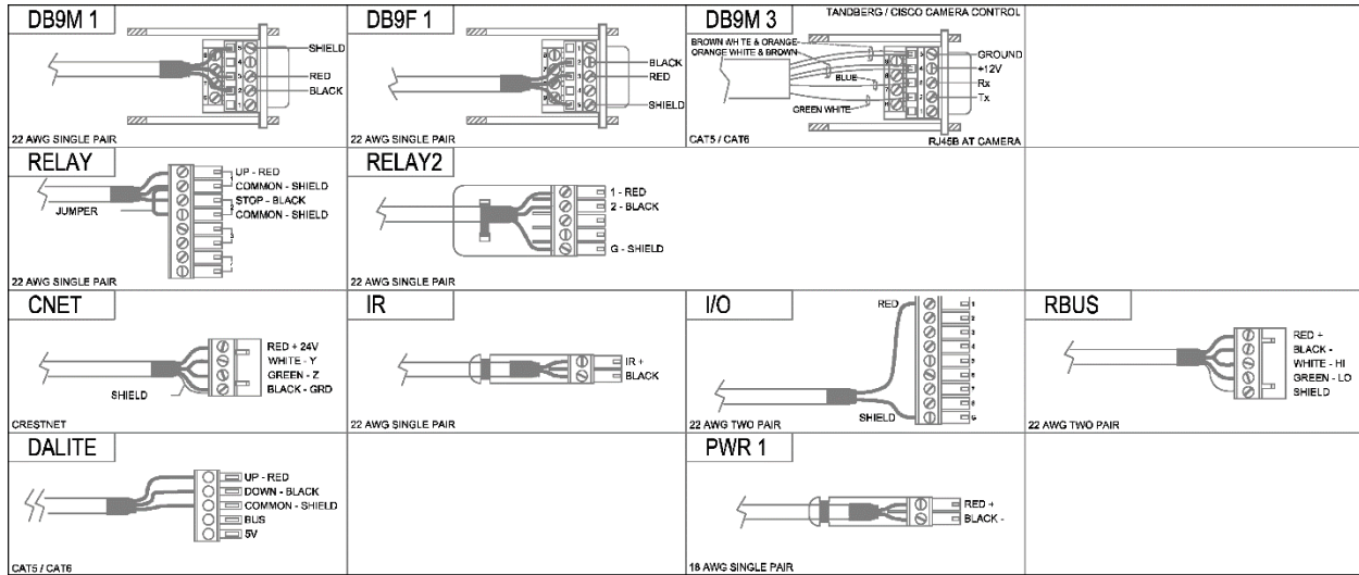
CABLING TABLE
